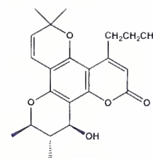
Calanolide A
